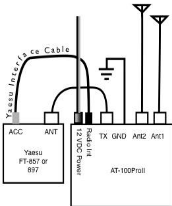
FT-857/897 Installation
