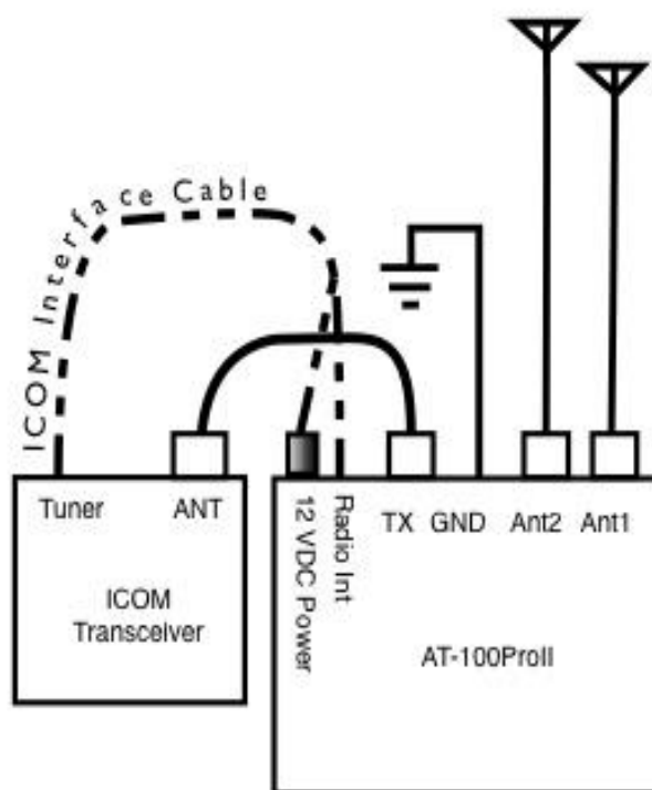
ICOM Installation
