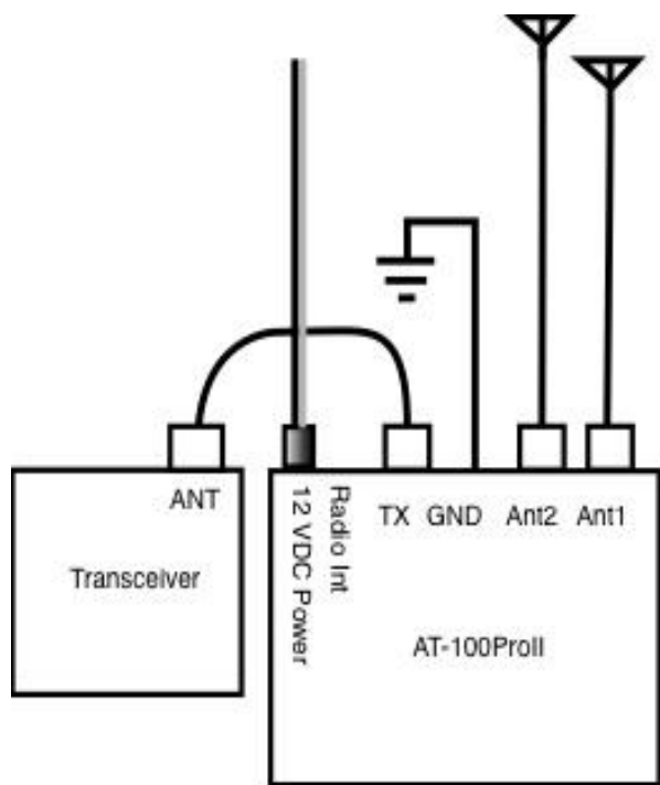
Typical Installation
